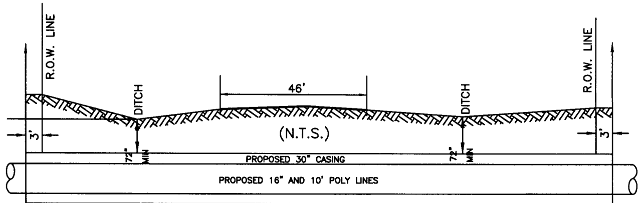
PLAN AND PROFILE OF 16" AND 10" POLYLINES & A 30" STEEL CASING
