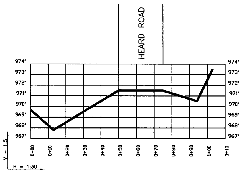
PLAN AND PROFILE OF 16" AND 10" POLYLINES & A 30" STEEL CASING
