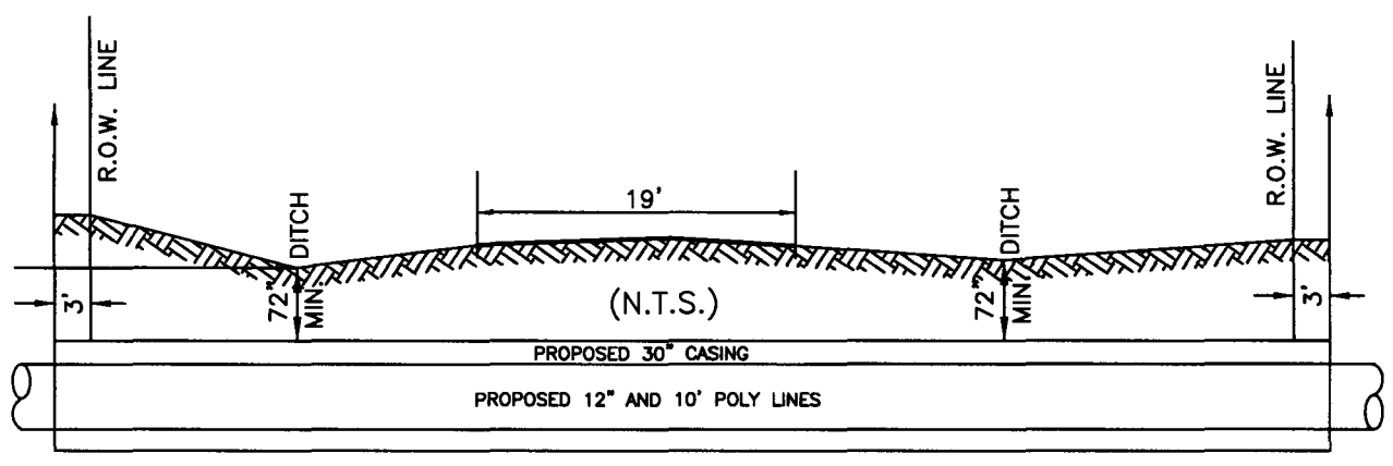
PLAN AND PROFILE OF A 30" STEEL CASING & 12" AND 10" POLYLINES
