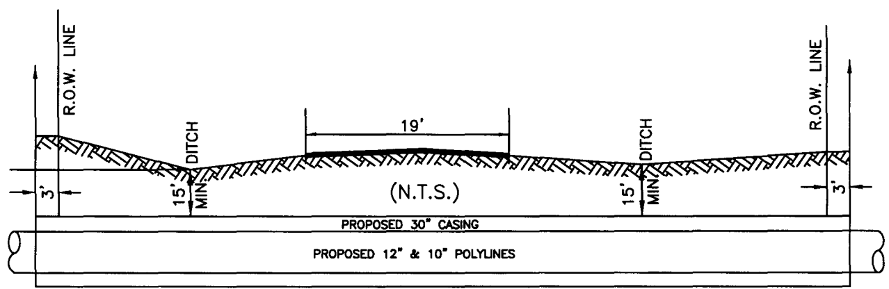
PLAN AND PROFILE OF A 30" STEEL CASING WITH 12" AND 10" POLYLINES
