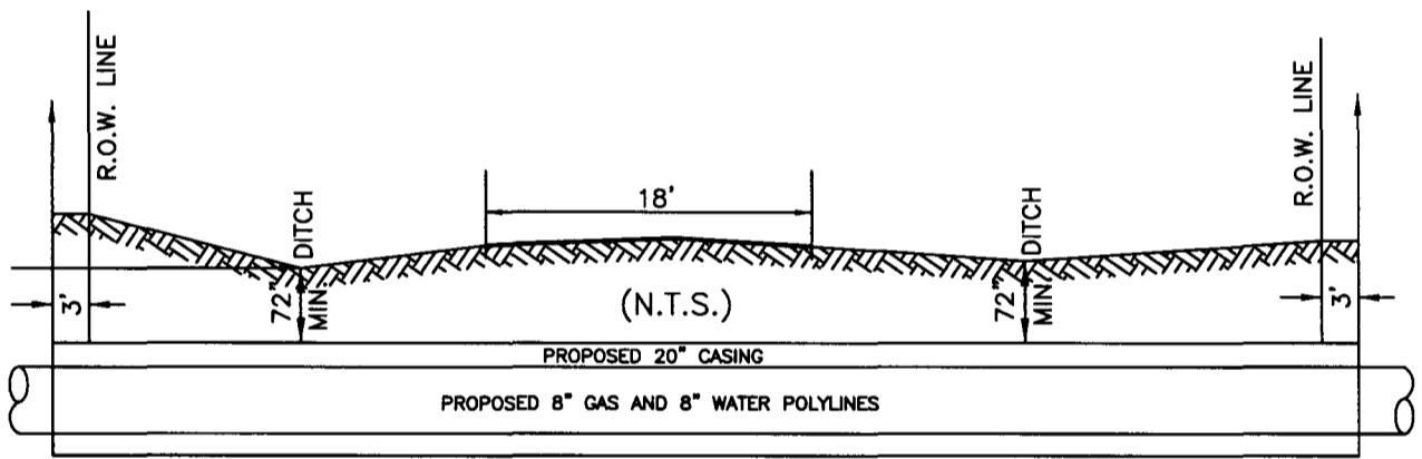
PLAN AND PROFILE OF 8" GAS AND 8" WATER POLYLINES & A 20" STEEL CASING
